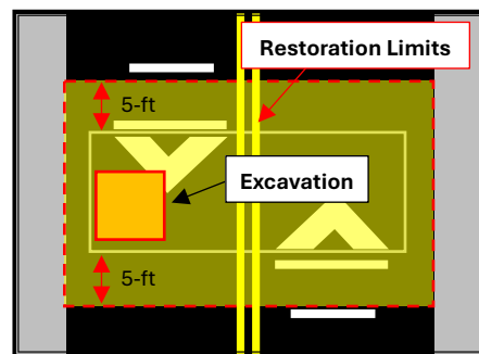
Restoration limits on a street with a speed hump/table
